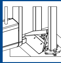
lower beam detailed view of slam support panel
